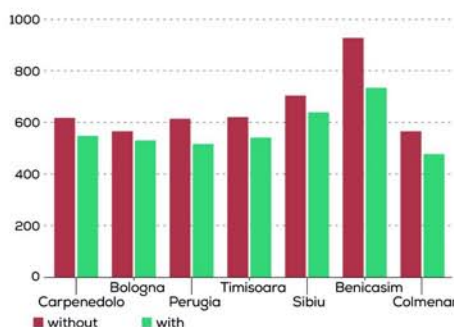
CO 2 e emissions in the different pilot stores by means of LCCP without and with Life-C4R technologies. Total impact assessment (kg CO 2 e per kWh)
